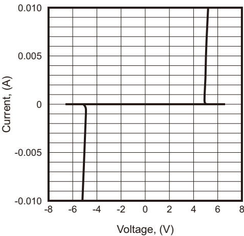
Fig.3 - Voltage Sweeping
