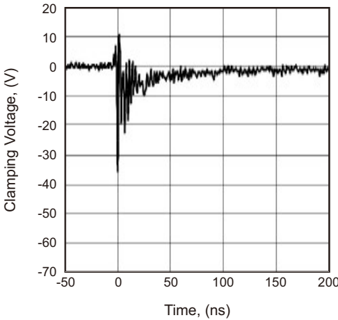
Fig.6 - ESD Clamping (-8kV Contact per IEC 61000-4-2)
