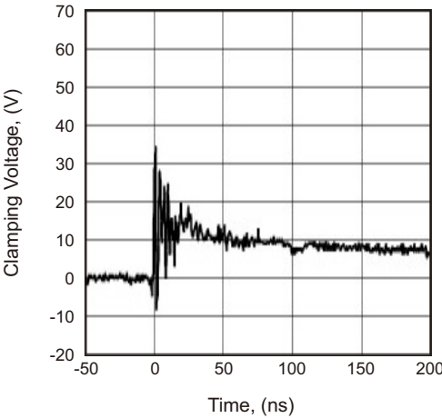
Fig.5 - ESD Clamping (+8kV Contact per IEC 61000-4-2)
